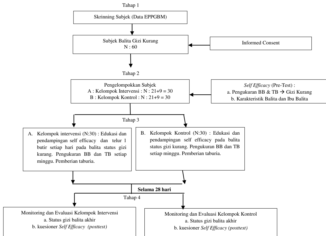
Gambar 2. Alur Penelitian
