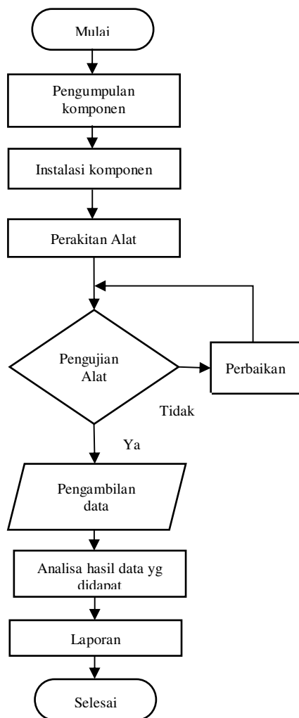
Gambar 1. Alur Penelitian.
