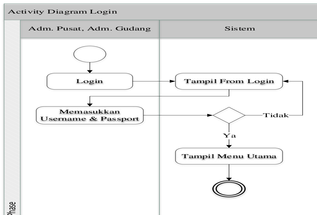
Gambar 4. Activity Diagram Login
