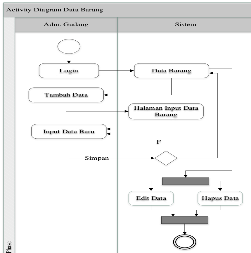
Gambar 3. Activity Diagram Data Barang
