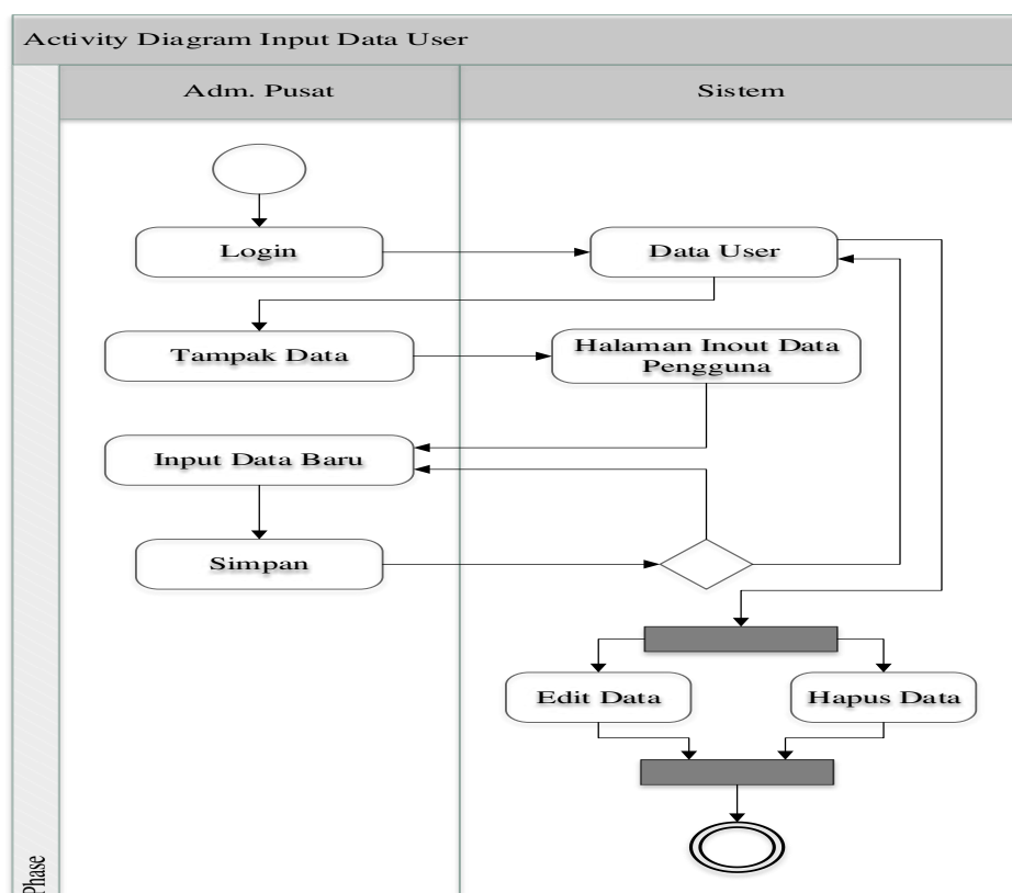
Gambar 5. Activity Diagram Data User
