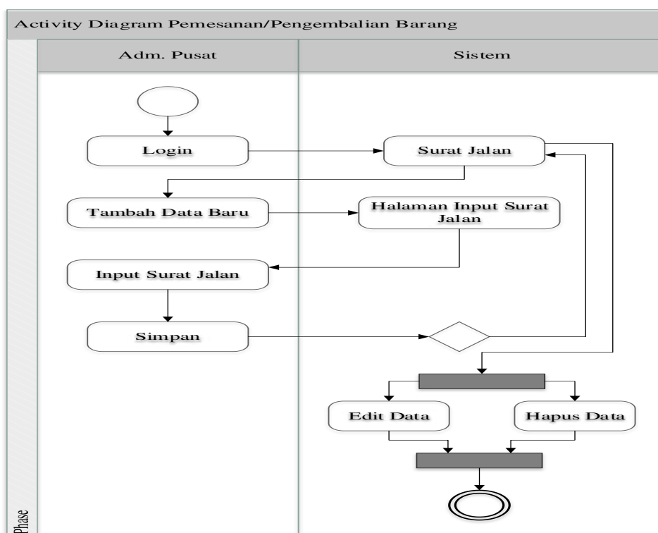
Gambar 6. Activity Diagram Mengelola Data Barang
