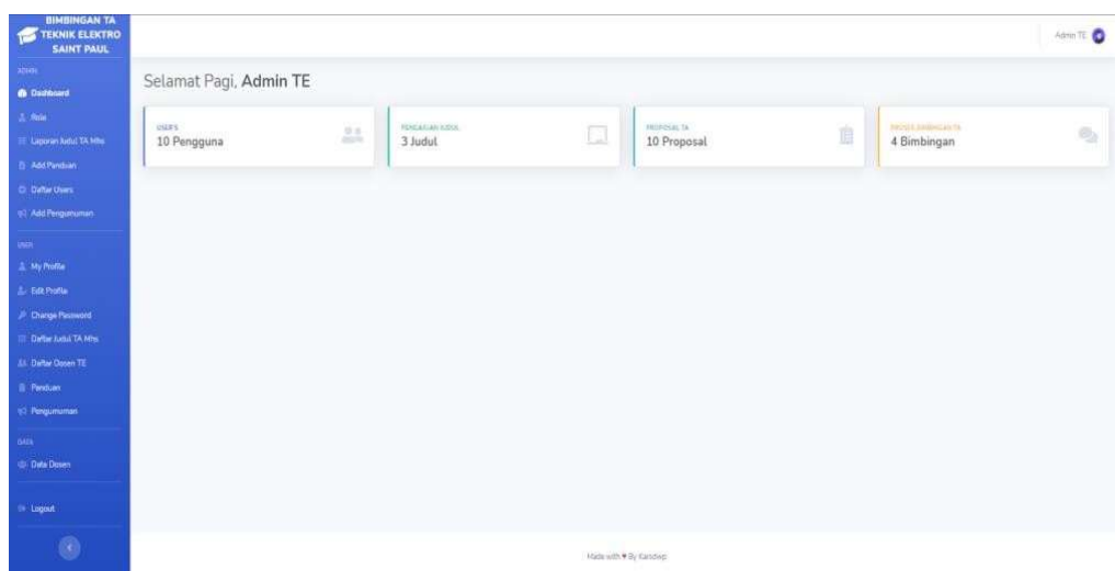
Gambar 4. Menu Dashboard
