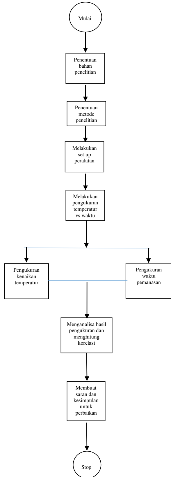
Gambar 3. Alur Penelitian
