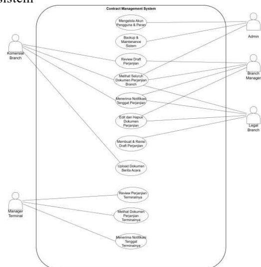
Gambar. 2 Use Case Diagram Setiap Role
