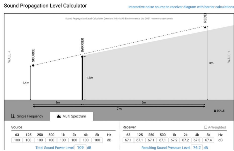
Gambar 5. Simulasi Noise Tools
