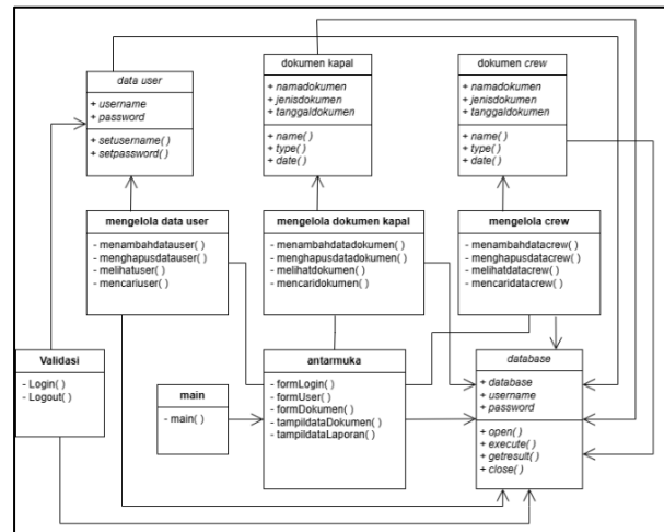
Gambar 7. Class Diagram
