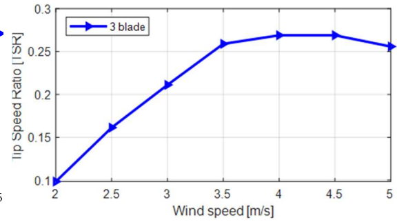
Figure 11. Tip Speed Curve Ratio to wind speed
