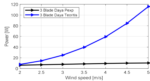
Figure 12. Theoretical and actual power curves against wind speed
