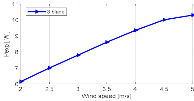
Figure 7. Actual power curve against wind speed
