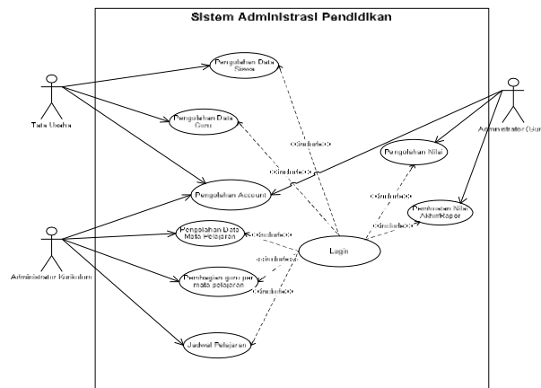
Gbr 1 UseCase Diagram input nilai
