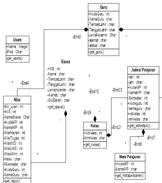
Gbr 2 Class Diagram
