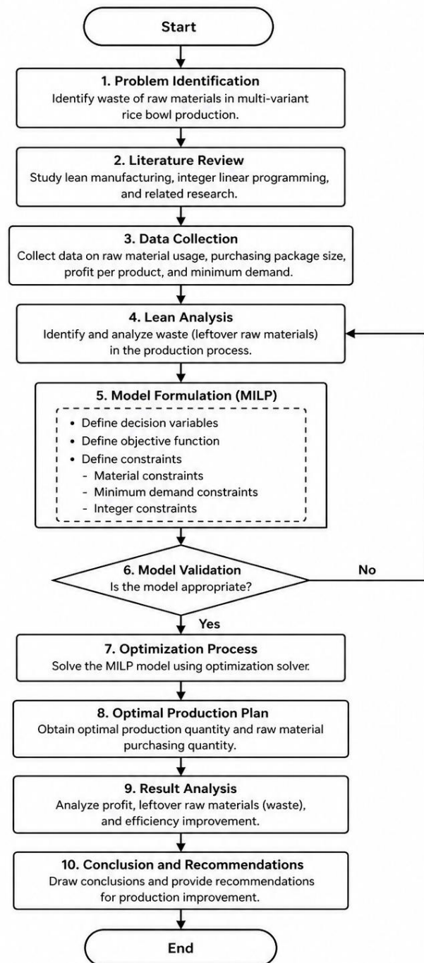
Figure 2. Metodologies Flowchart
