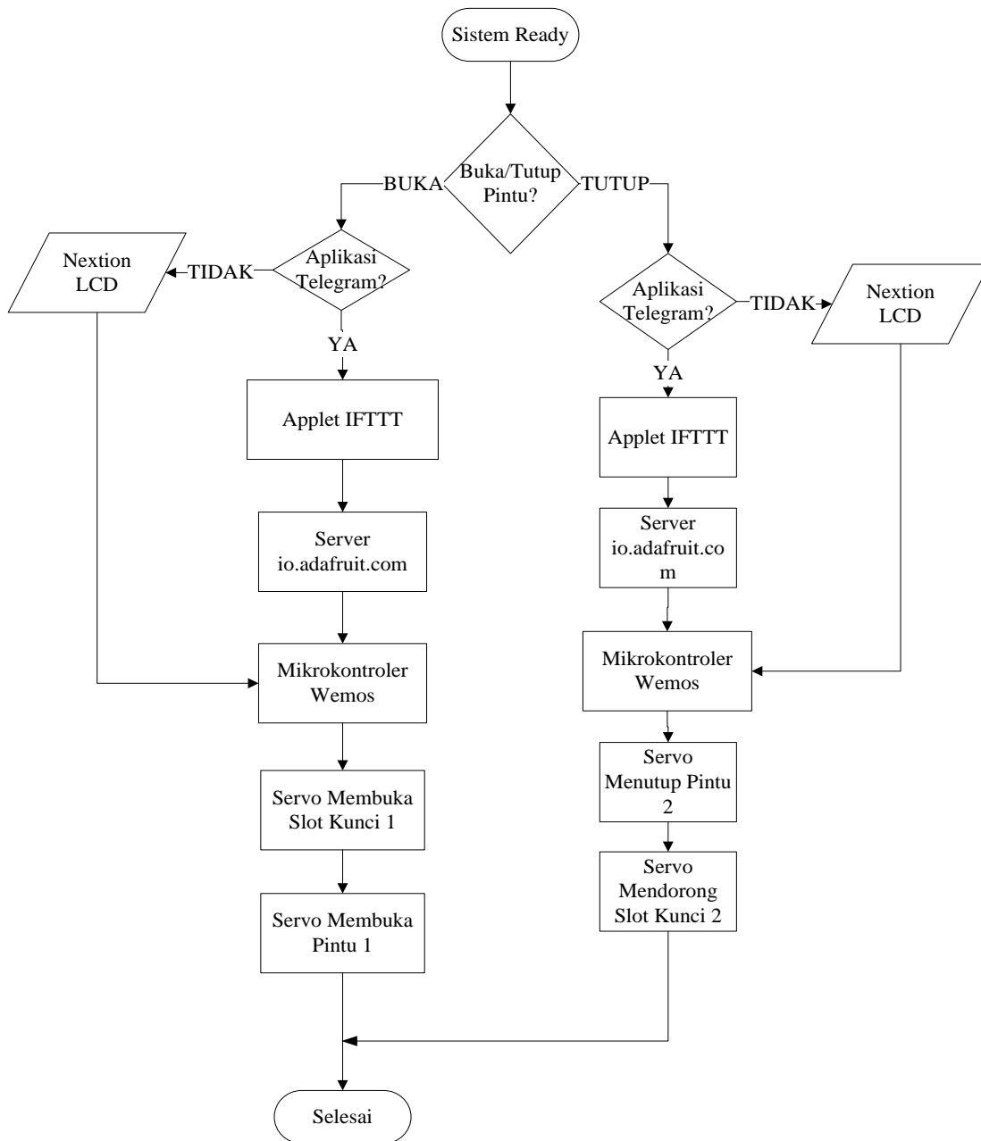
Figure 3. Door Control System Workflow
