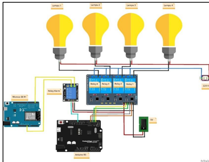
Figure 5. Relay Circuit Lights and Alarms
