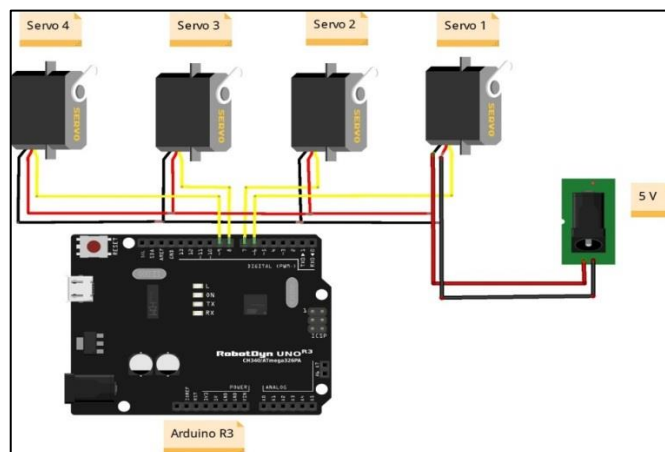
Figure 6. Servo Suite
