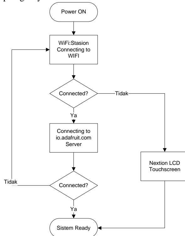
Figure 2. How The System Workflow Works
