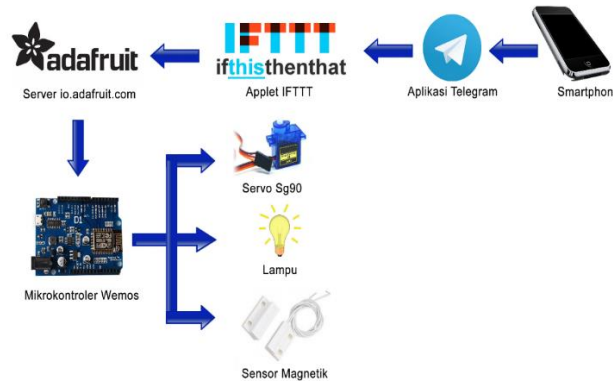
Figure 1. Diagram of How the System Works
