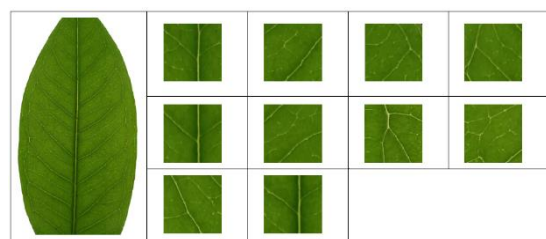
Figure 4. Image Cropping
