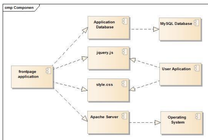
Gambar 12: Component Diagram
