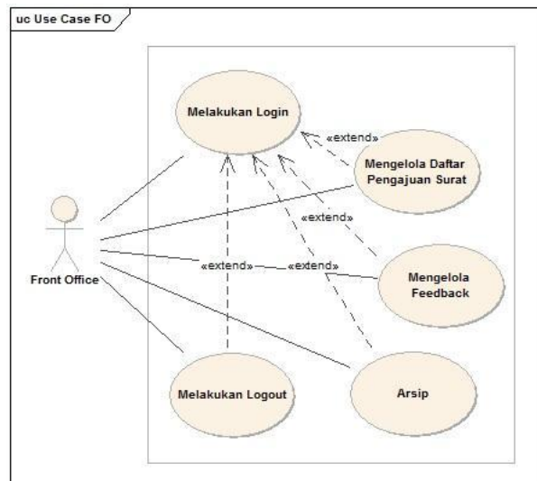
Gambar 3: Usecase Diagram Front Office
