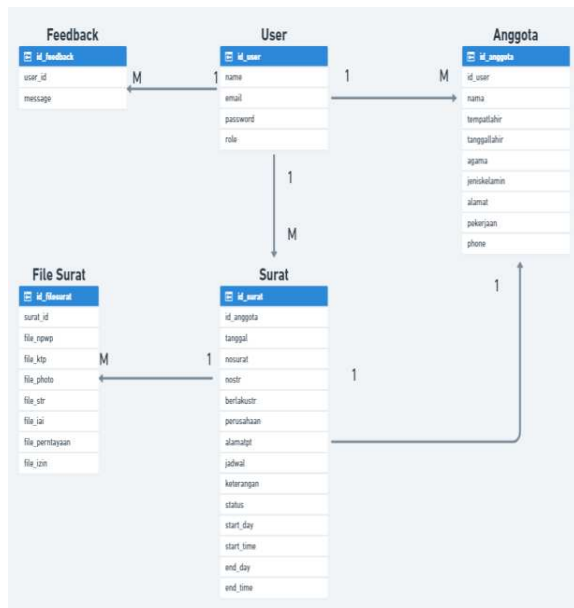
Gambar 11: Logical Record Structure (LRS)
