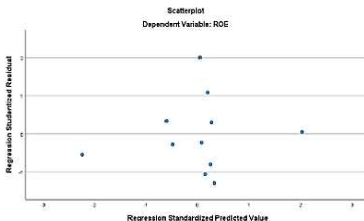
Gambar 3. Scatterplot
