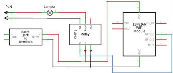
Figure 6. Installation Scheme of ESP01S and Relay
