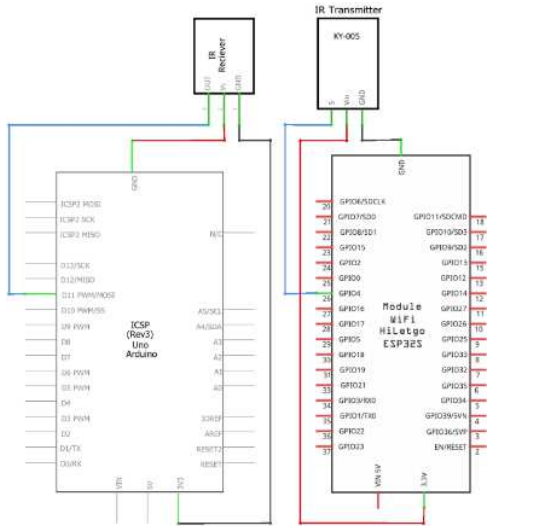
Figure 7. Installation Scheme of IR Transmitter and Receiver
