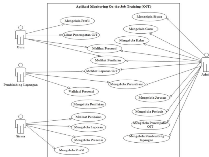
Gambar 2. Use Case Monitoring Praktek Kerja Industri
