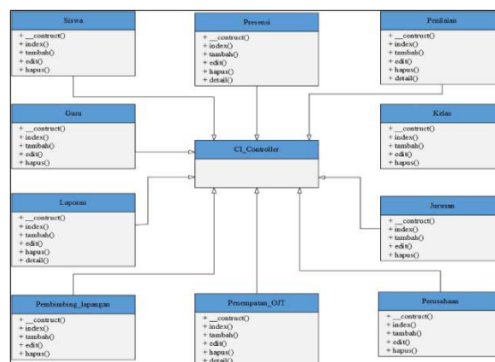
Gambar 3. Class Diagram Controller
