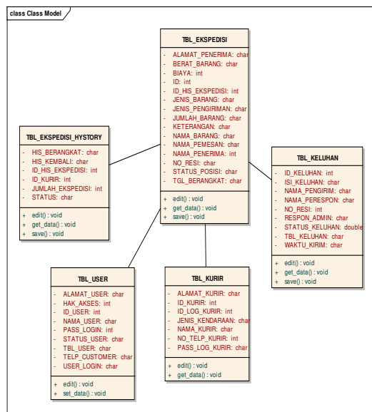
Gambar 5. Class Diagram
