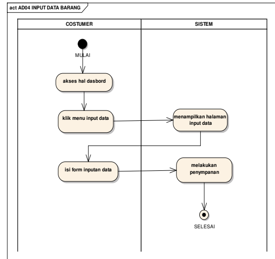
Gambar 3. Activity Diagram Input Data Barang
