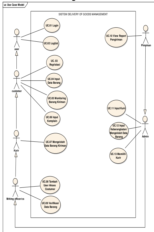
Gambar 2. Use Case Description
