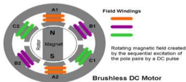
Figure 3. Brushless Direct Current Motor Source: author 2022
