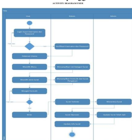
Gambar 3. Activity Diagram
