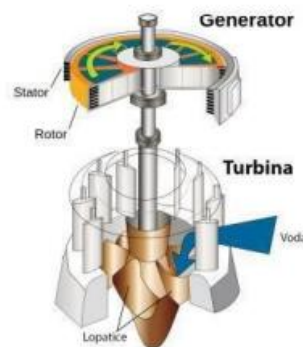
Gambar 3 Turbin Kaplan (Sofyan & Sudana, 2022)
