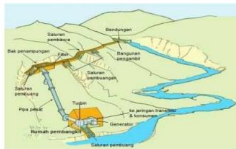
Gambar 2 Skema PLTMH (Sofyan & Sudana, 2022)
