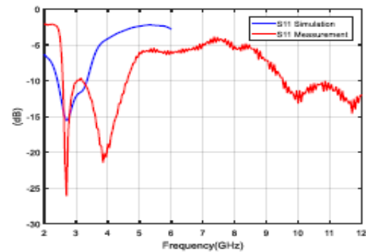
Gambar 15. Perbandingan Return Loss
