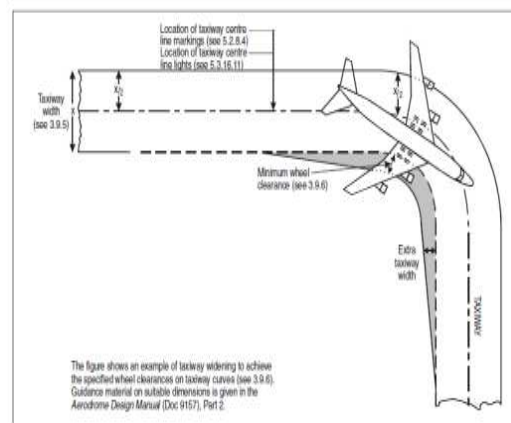
Gambar 1. Exit taxiway
