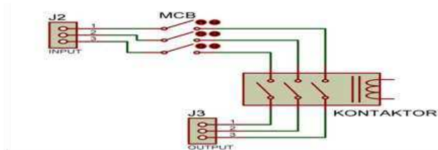
Figure 5. MCB circuit
