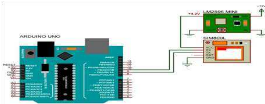
Figure 2. Sim800L Series
