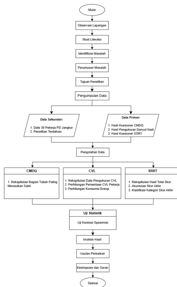
Gambar 1. Flowchart Penelitian
