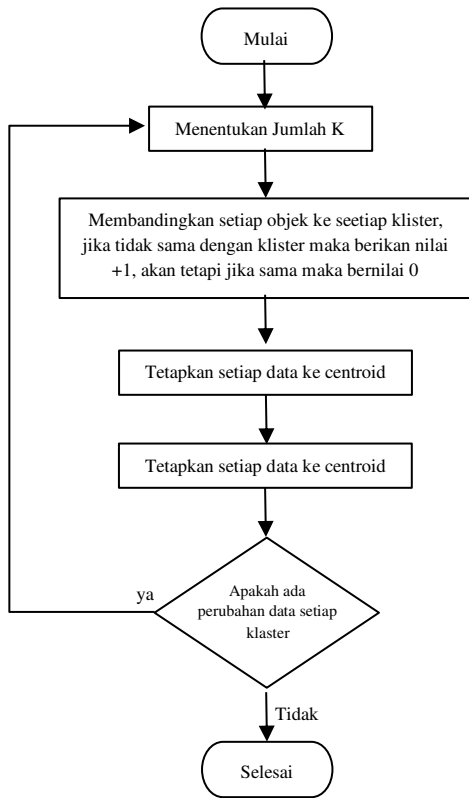
Gambar 1. Flowchart K modes
