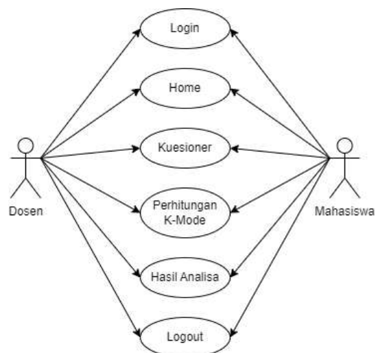
Gambar 3. Use case sistem K modes
