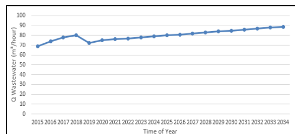
Figure 5. Terminal 3 Wastewater Generation from 2015 to 2034
