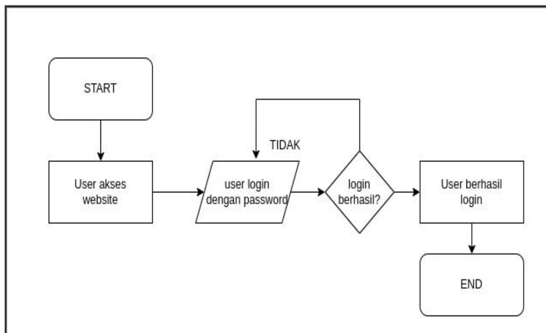
Figure 2 Flowchart Login
