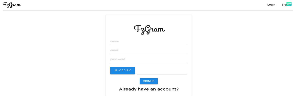
Figure 7 Halaman Register
