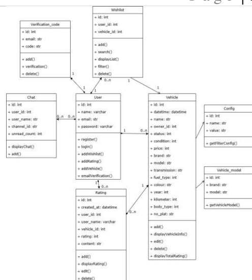
Gambar 5. Class Diagram
