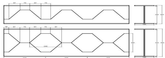
Gambar 1. Geometri Penampang Baja Castella IWF450.150.6,5.9
