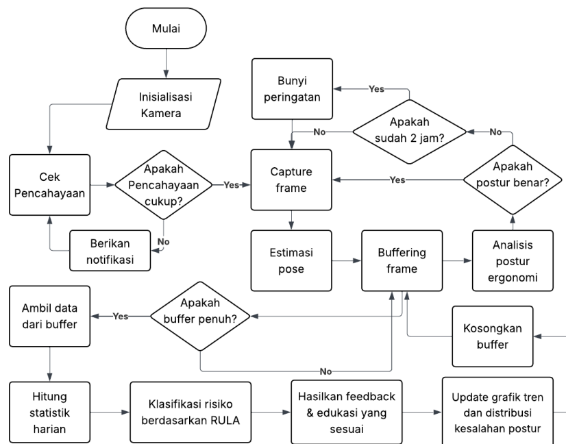
Gambar 1. Alur sistem K-POSE
