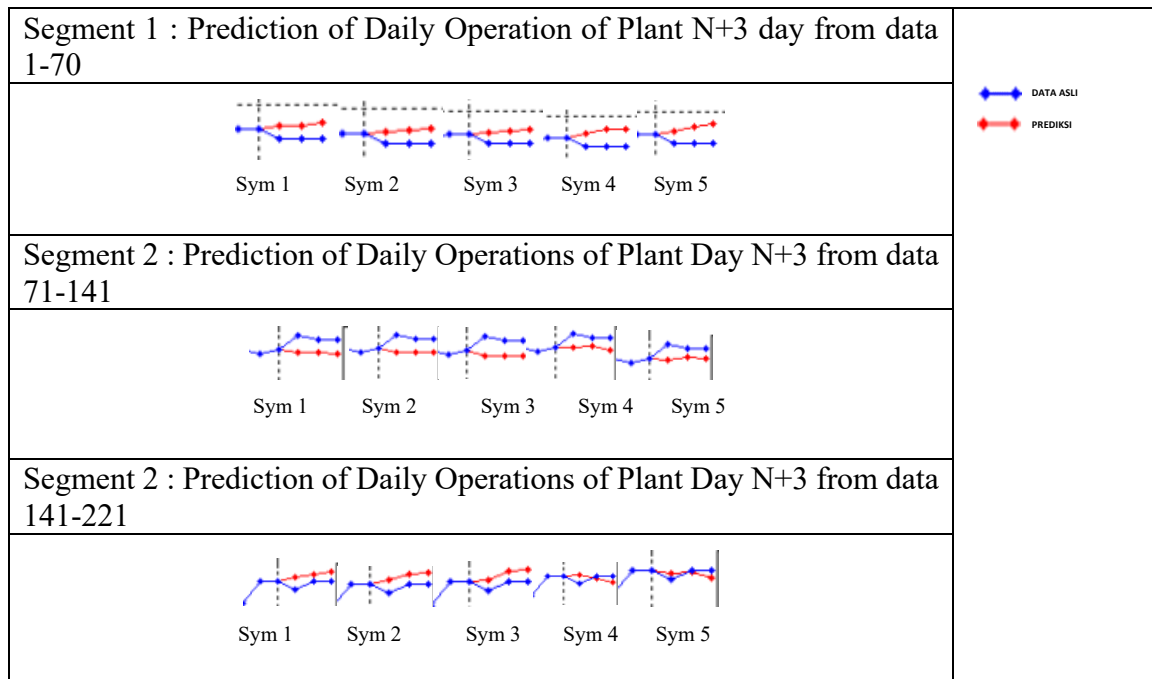
Figure 2. Prediction results in each segment of the plant's daily operation data
