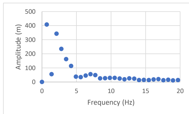
Figure 2. FFT of the sea level at Maumere over period of January 12-14, 2024
