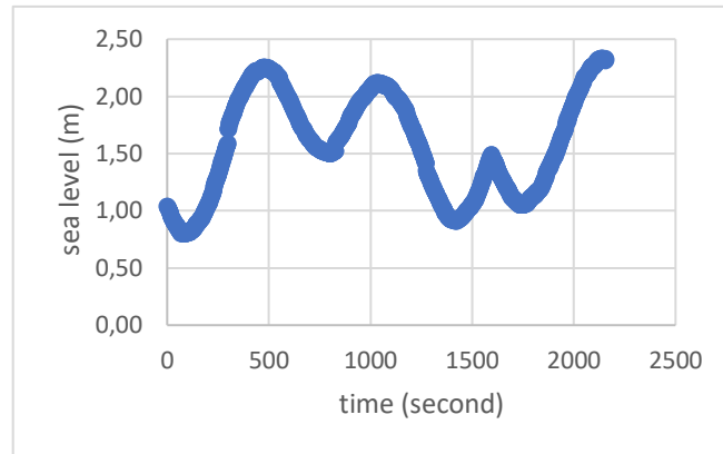
Figure 1. Graph of the sea level at Maumere over period of January 12-14, 2024
