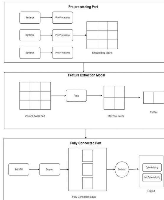
Gambar 3. Arsitektur Hybrid Learning Model
