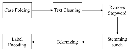
Gambar 4. Preprocessing
