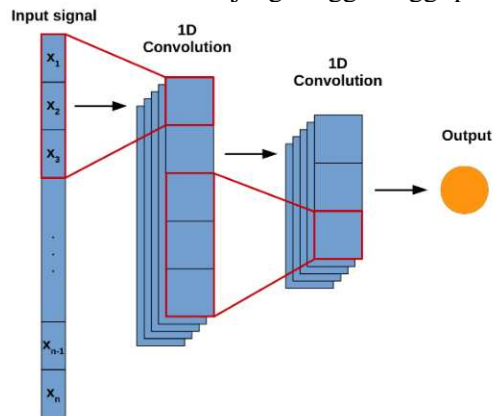
Gambar 2. 1D CNN Architecture
