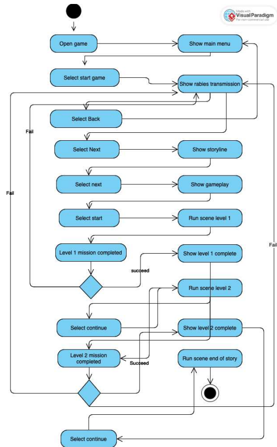
Figure. 4. Activity Diagram
