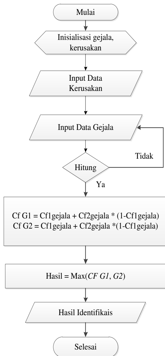
Gambar 1. Flowchart Metode
