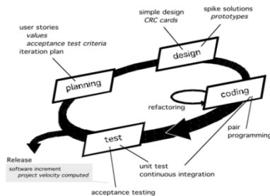
Gambar 2. Extreme Programming
