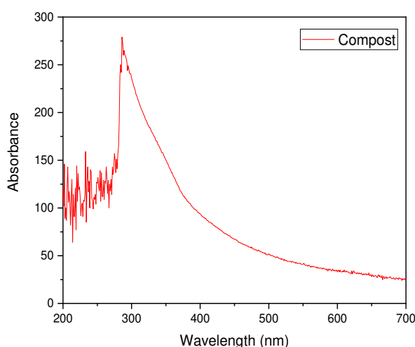
Figure 2. The UV-Vis spectrum of Humic Acid
