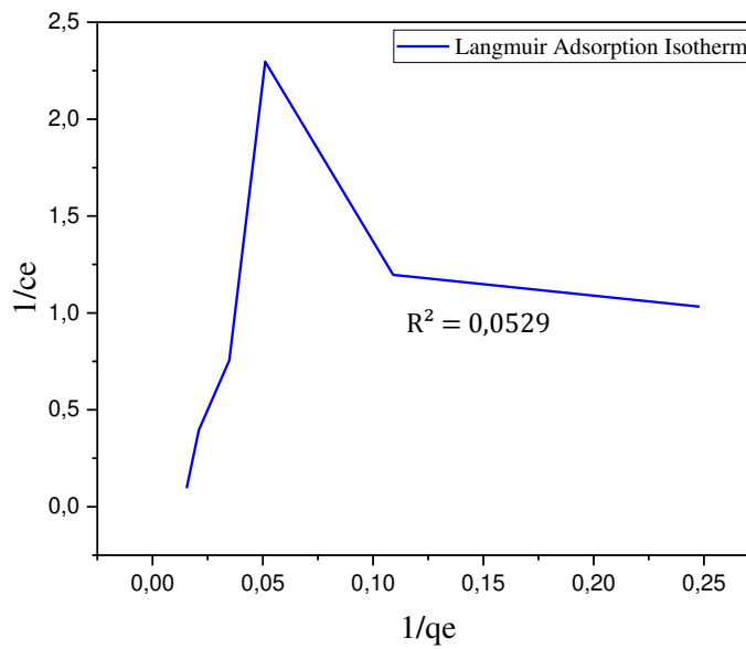
Figure 9. Langmuir Adsorption Isotherm Graph
