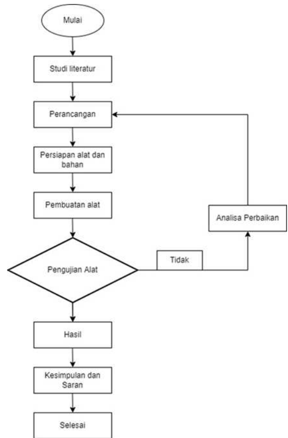
Gambar 1. Alur Penelitian
