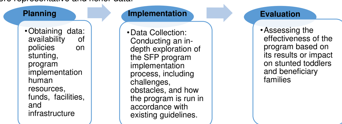
Figure 1. Research Stage
