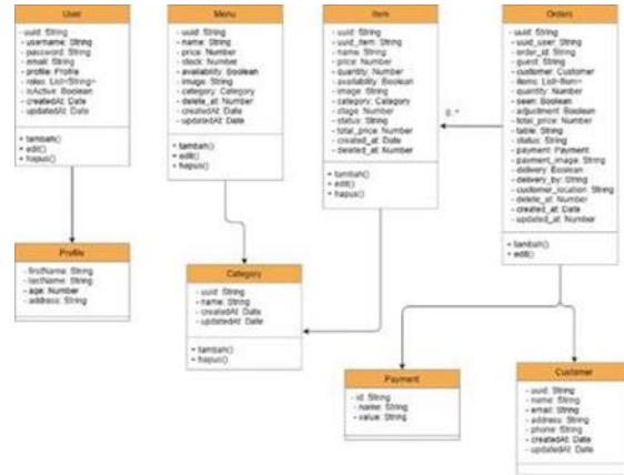
Gambar 3.2.1 Class Diagram
