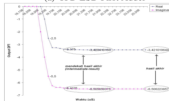
(b) TFD MSB-First Adder
