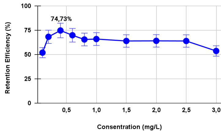
Figure 4. Effect of initial Cr(VI) concentration on the retention efficiency of Ca-Alg-EDTA microcapsules (n=3, pH 2 \pm 0.5 , contact time 24 h).
