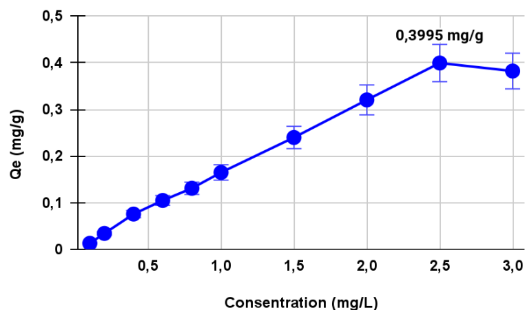
Figure 5. Effect of initial Cr(VI) concentration on the retention capacity of Ca-Alg-EDTA microcapsules (n=3, pH 2 \pm 0.5 , contact time 24 h).
