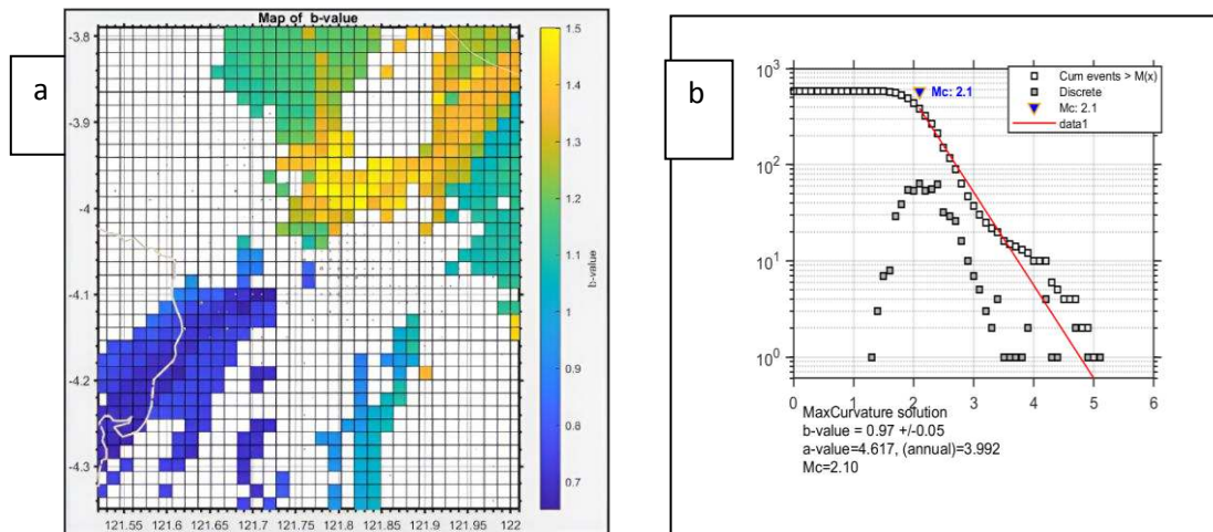
Figure 2. (a) Map of spatial variation of the seismic b-values in the East Kolaka and surrounding areas. (b) Graph of M_c (Magnitude Completeness) values, b-values and a-values in East Kolaka and surrounding areas. Plotted are both the cumulative (red line) and non-cumulative (outside the red line) forms.
