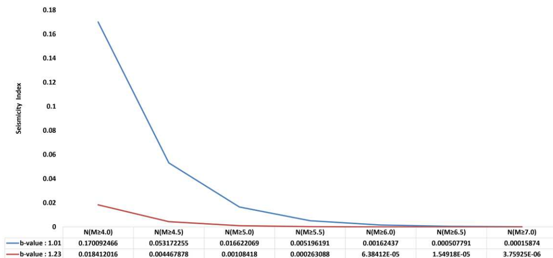
Figure 7. Seismicity index values for earthquakes with M \geq 4.0 , M \geq 4.5 , M \geq 5.0 , M \geq 5.5 , M \geq 6.0 , M \geq 6.5 , and M \geq 7.0 in the cross-section AA' region, based on the minimum (blue line) and maximum (red line) b-values.
