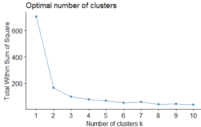
Gambar 2 Penentuan K-Optimum
