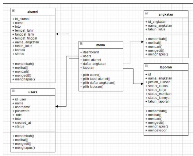
Gambar 4. 3. Class Diagram
