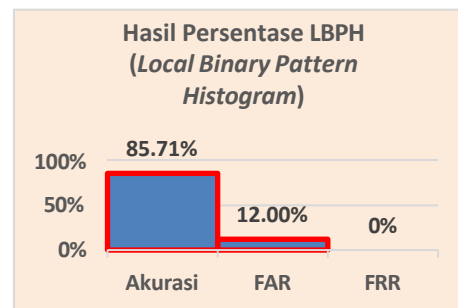
Gambar 3.6.4 Grafik Persentase LBPH ( Local Binary Pattern Histogram )
