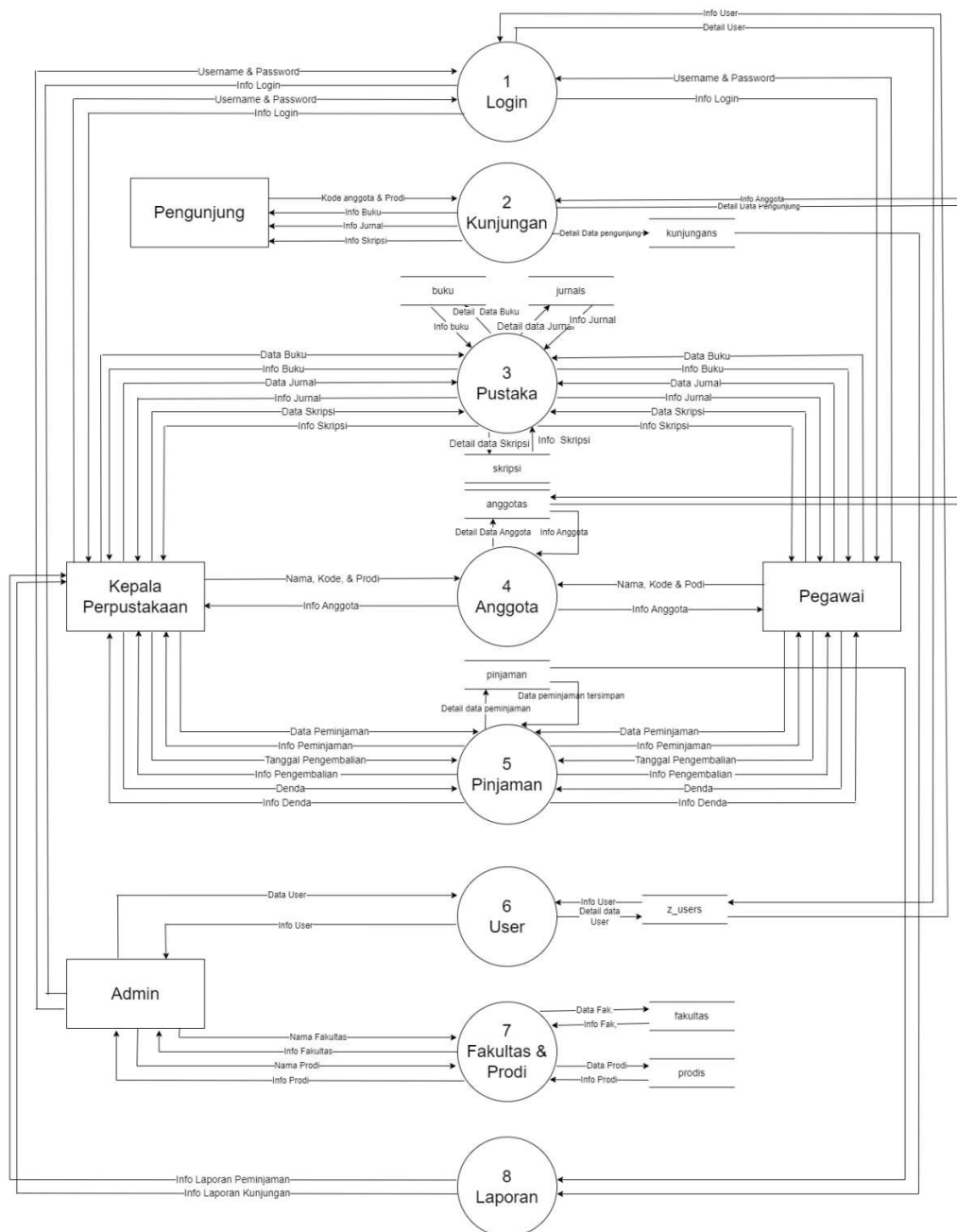
Gambar 3. Data Flow Diagram Sistem
