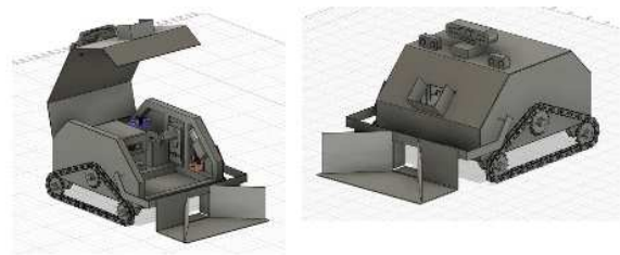
Gambar 7 Mechanical Design
