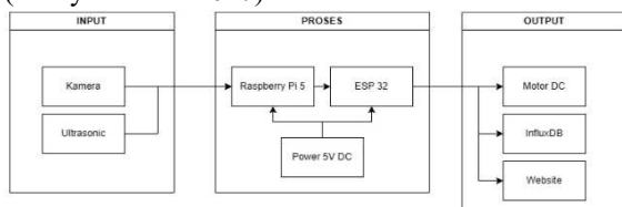
Gambar 3 Blok Diagram
