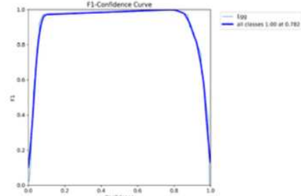
Gambar 14 F1-Confidence Curve
