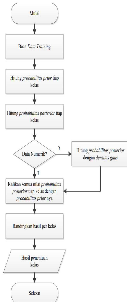
Gambar 1. Alur Metode Naïve Bayes Classifier
